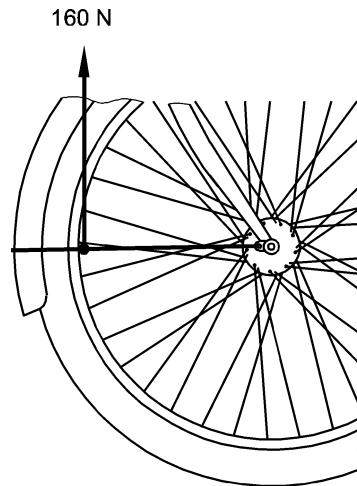
Figure 35 — Front mudguard: tangential obstruction test
