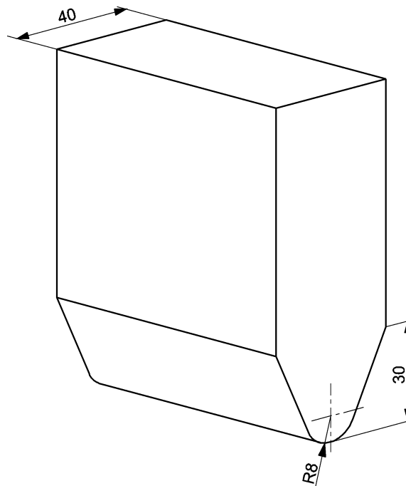
Figure 39 — Striker dimensions
