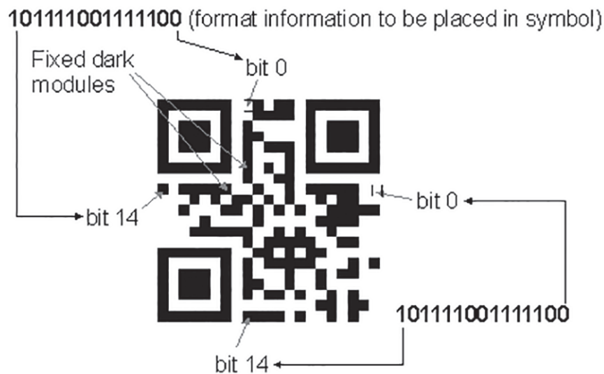
Figure I.2 — Final version 1-M symbol encoding 01234567
